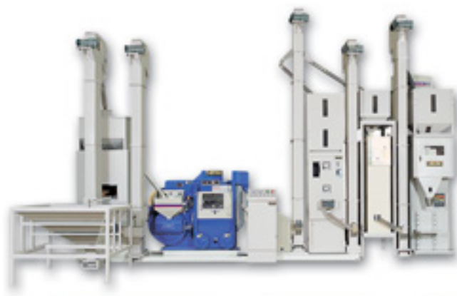
Grain selection assembly 벼정선부 Hulling assembly 현미부 Polishing assembly 정미부 Sorting assembly 색채 선별부 Measuring and packing assembly 계량포장부
